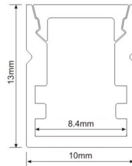
DIMENSIONS (MM)
