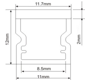
DIMENSIONS (MM)
