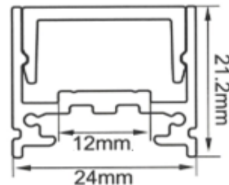
DIMENSIONS (MM)
