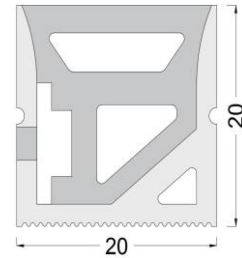
DIMENSIONS (MM)
